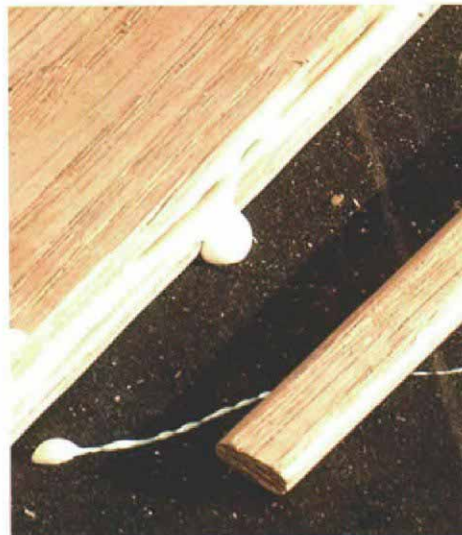
Reverse the flooring's direction with a slip tongue. Lengths of hardwood splines are glued and pinned into the groove of a center starter course. The flooring can then be nailed down in the opposite direction.
