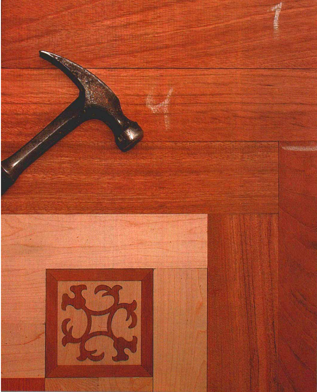
A temporary stop establishes the border's line. Screwed into the subfloor, scrap flooring provides a clean starting point for the flooring and a fast, straight line for one side of the floor's border.
